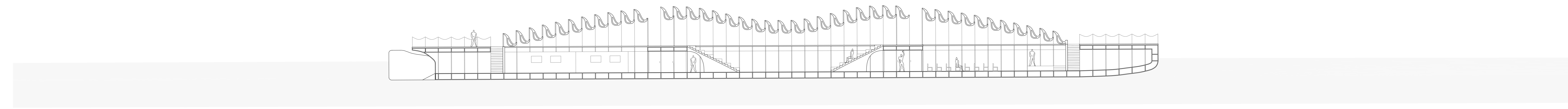
Section AA 1:200
